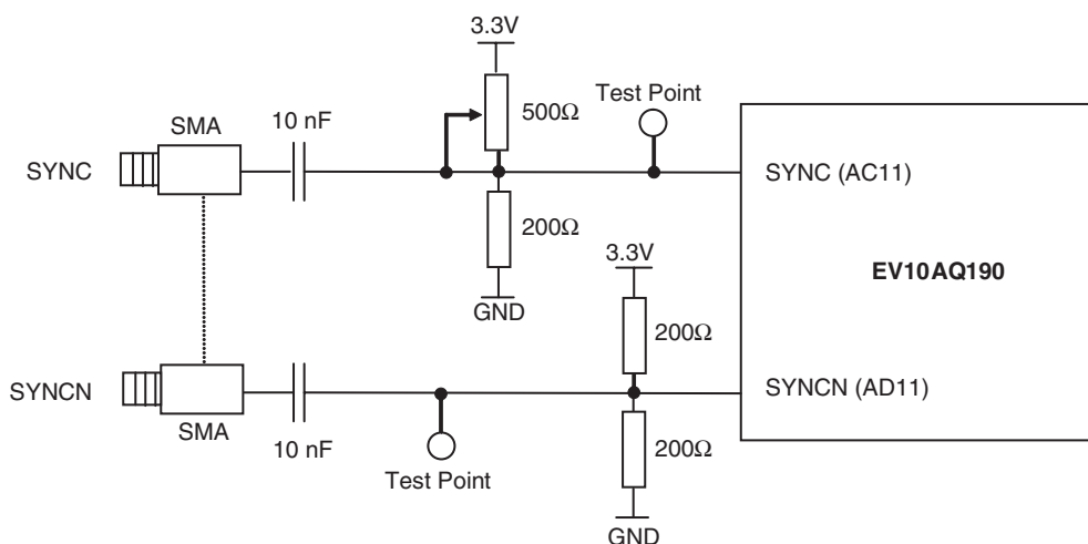
Figure 5-3. SYNCN, SYNCN Inputs Implementation
