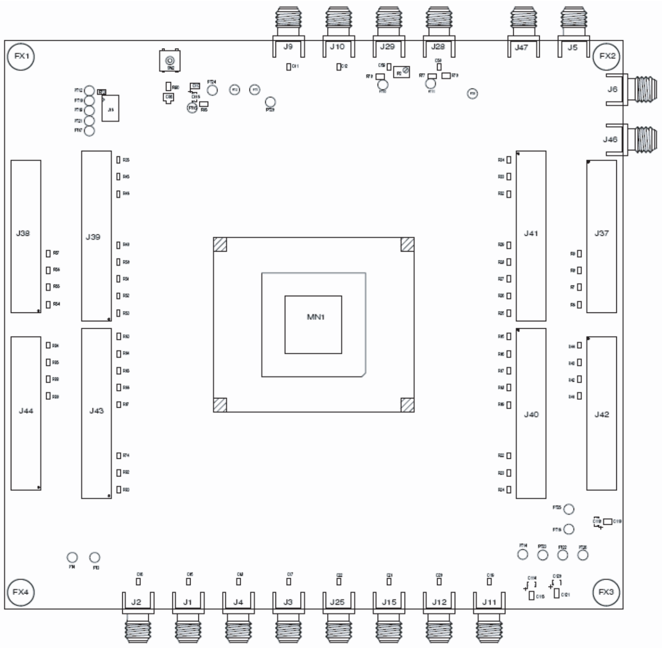
Figure 7-7. Equipped Board (Top)
