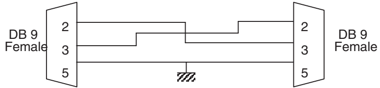
Figure 4-12. Crossed Cable
