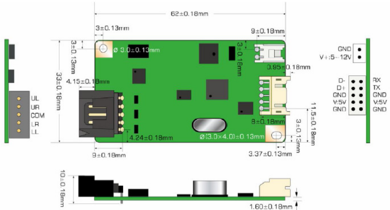
Figure 2: Pin Assignment
