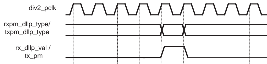
Figure 7. PM DLLP Transmit User Interface
