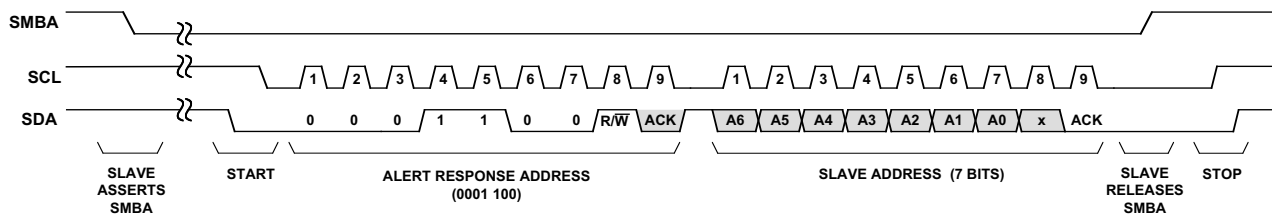
Figure 2-25. SMBAlert Bus Transaction
