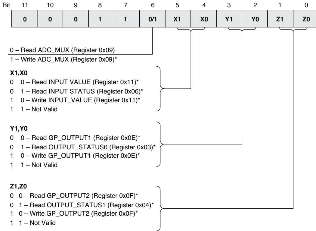
Figure 2-35. I2C_Control_Register
