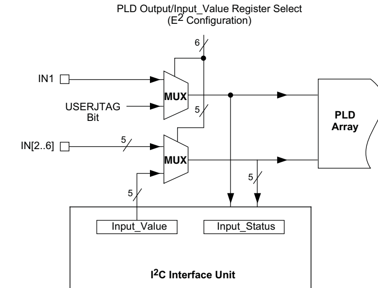
Figure 25. I 2 C Digital Input Interface
