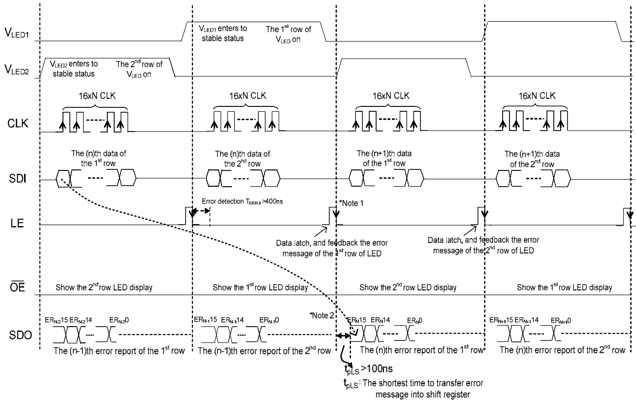
Figure 7. In-message error detection by \frac{1}{2} duty time-multiplexing circuit – error detection is triggered by LE
