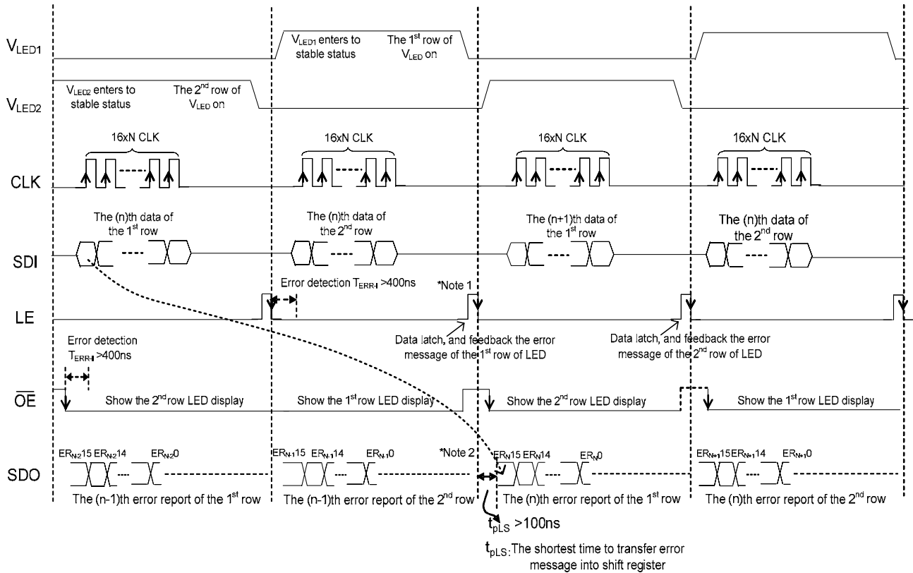
Figure 6. In-message error detection by \frac{1}{2} duty time-multiplexing circuit – error detection is triggered by LE or \overline{OE}
