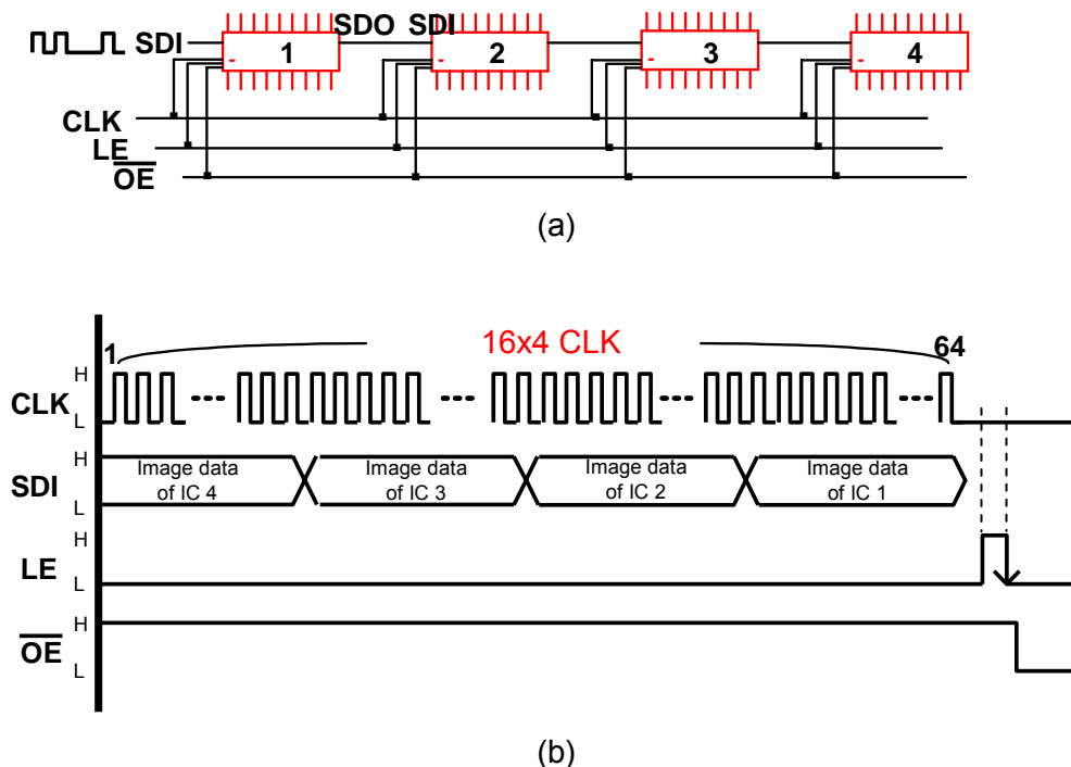
Figure 3(a). The sketch of 4pcs MBI5039 is in cascade. 3(b). The timing diagram of 4pcs MBI5039 is in cascade.
