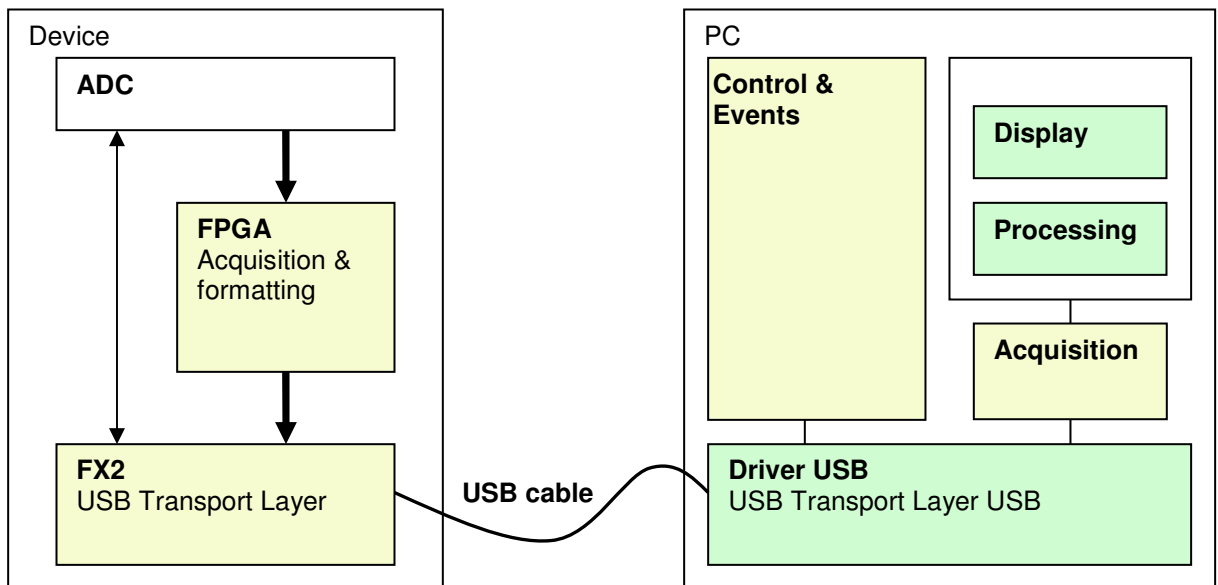
Figure 4. EV10AQ190TPY-DK Demo Kit functional architecture
