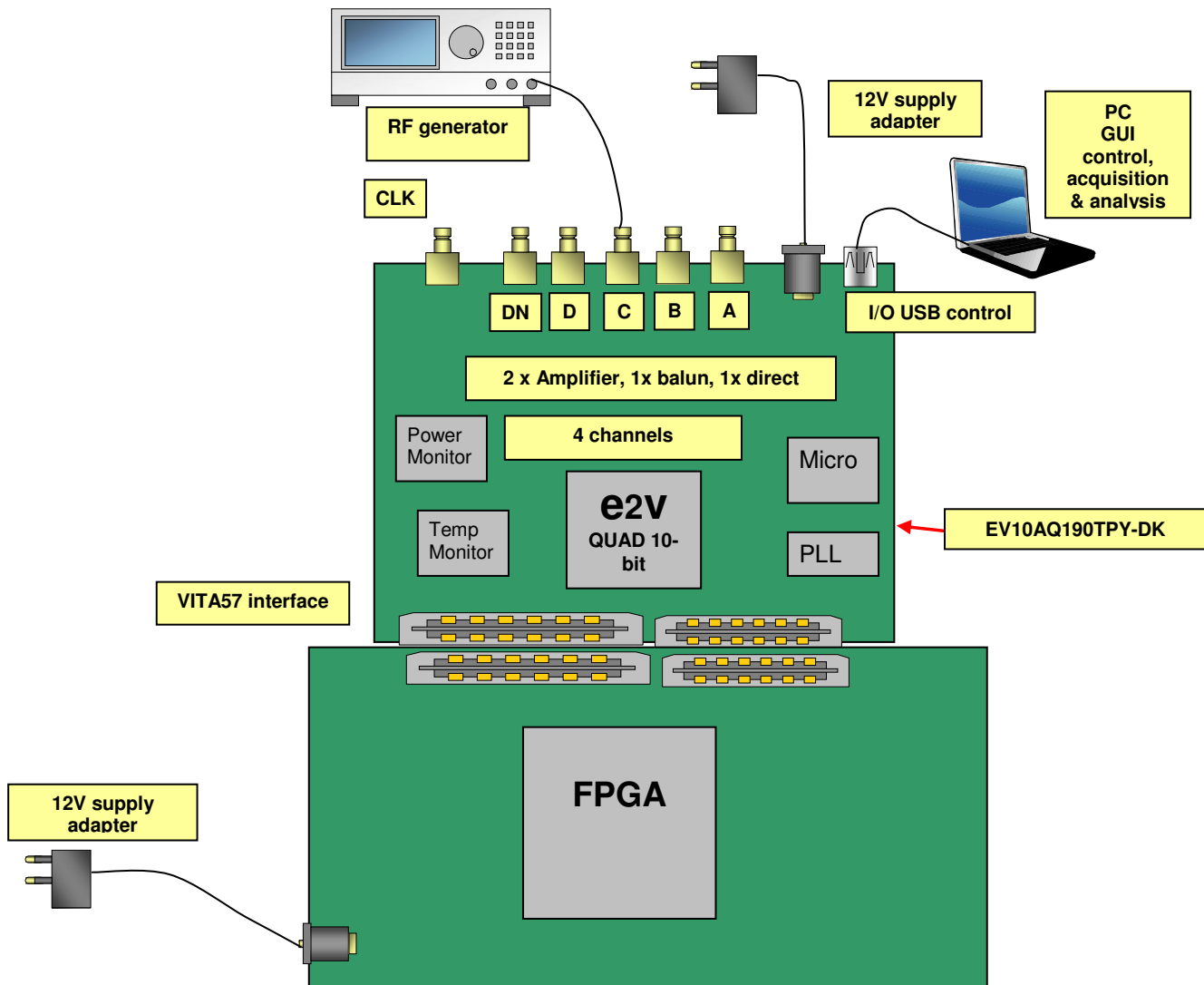
Figure 2. EV10AQ190TPY-DK Demo Kit system architecture (when connected with a VIRTEX6 Evaluation kit)
