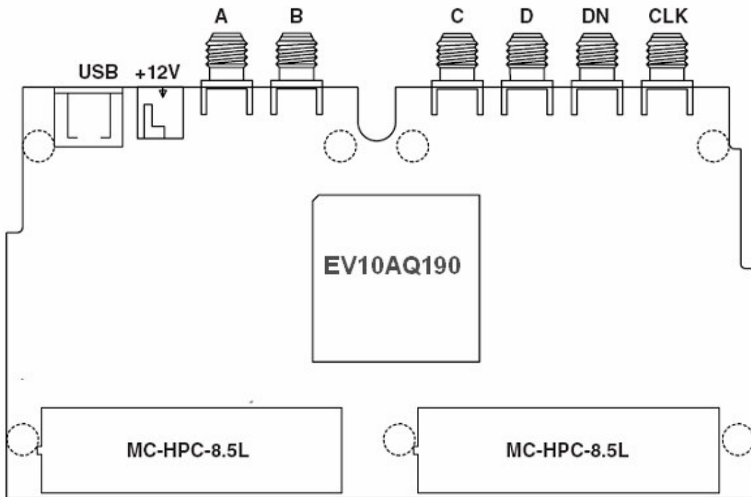
Figure 4. EV10AQ190TPY-DK Demo Kit functional architecture
