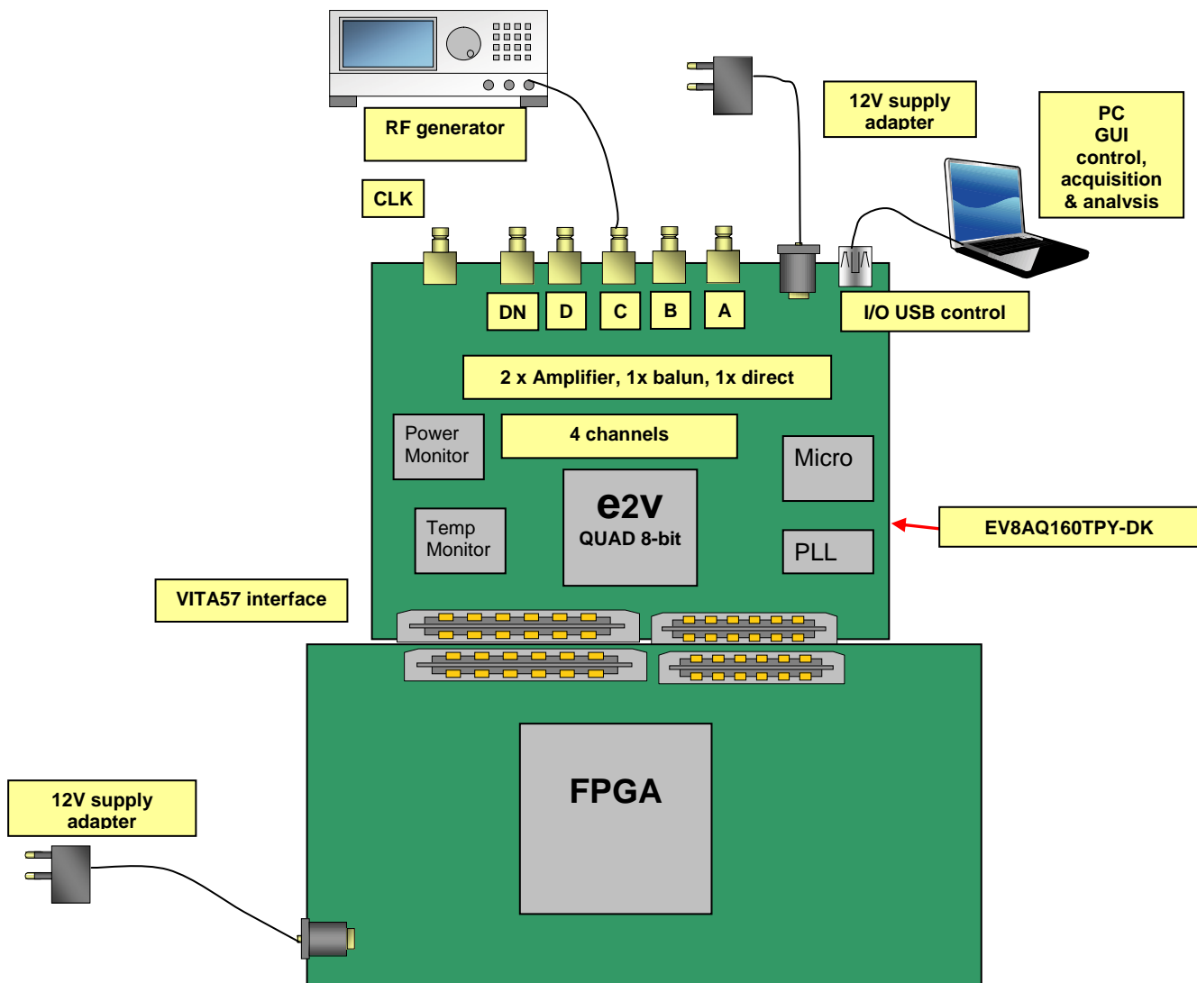
Figure 2. EV8AQ160TPY-DK Demo Kit system architecture (when connected with a VIRTEX6 Evaluation kit)
