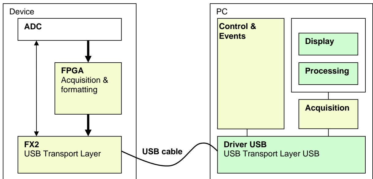
Figure 4. EV8AQ160TPY-DK Demo Kit functional architecture
