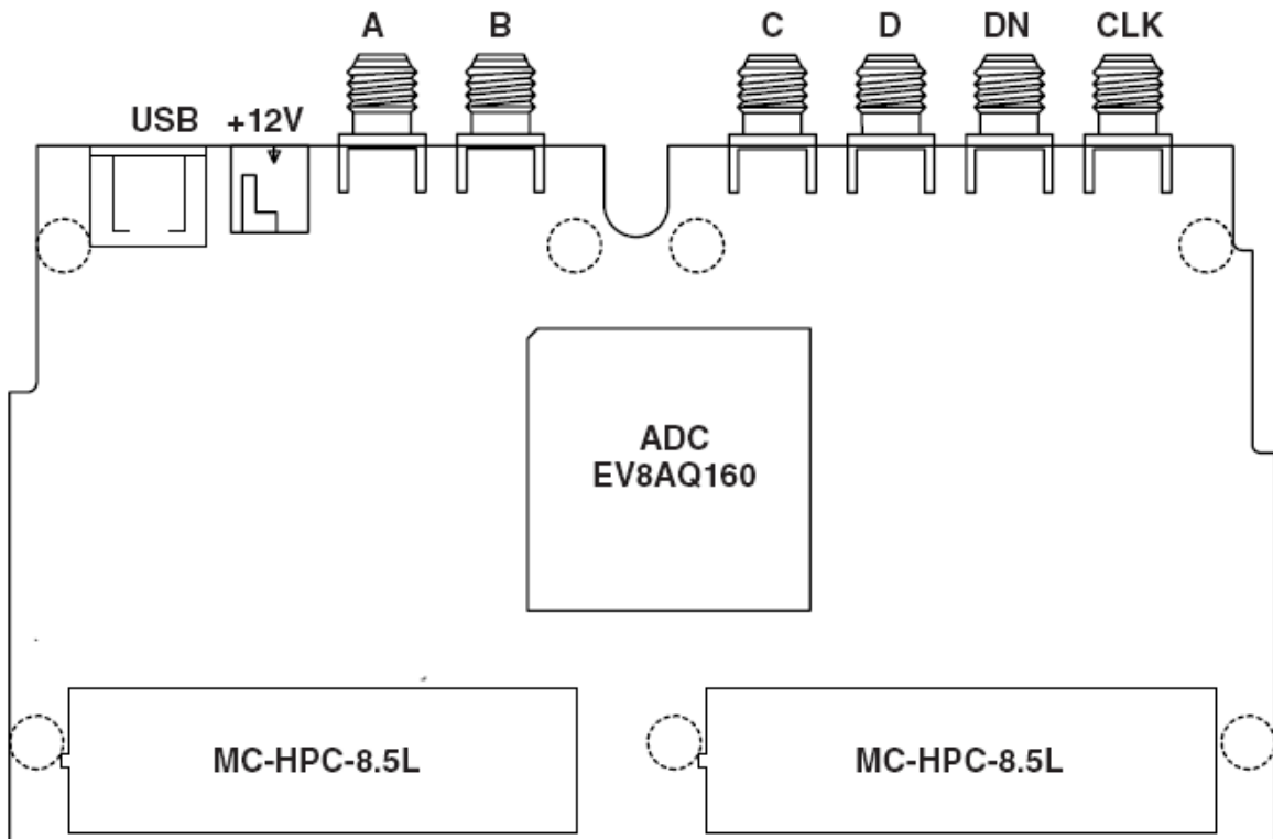
Figure 4. EV8AQ160TPY-DK Demo Kit functional architecture
