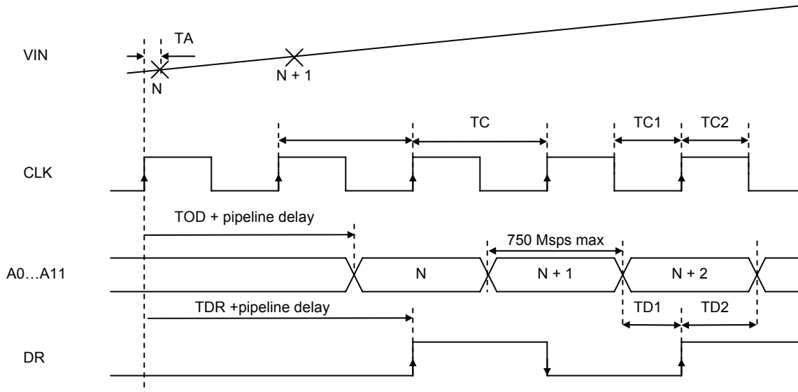
Figure 2 Principle of operation, DMUX 1:2
