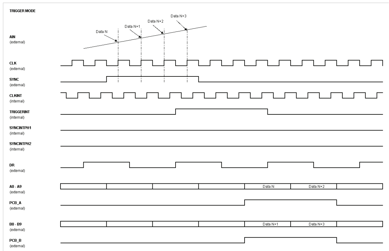
Figure 7 Trigger mode diagram
