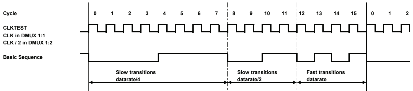
Figure 6 Alignment pattern timing diagram
