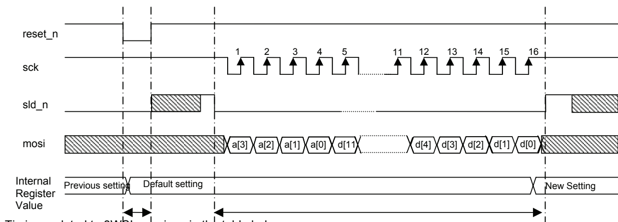
Figure 8 3WSI Timing Diagram
