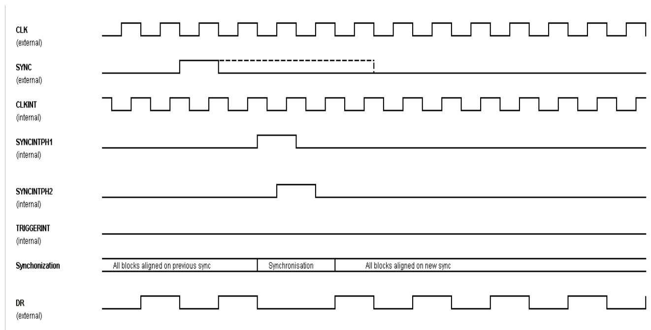
Figure 4 External reset Timing diagram (1:1 DMUX)
