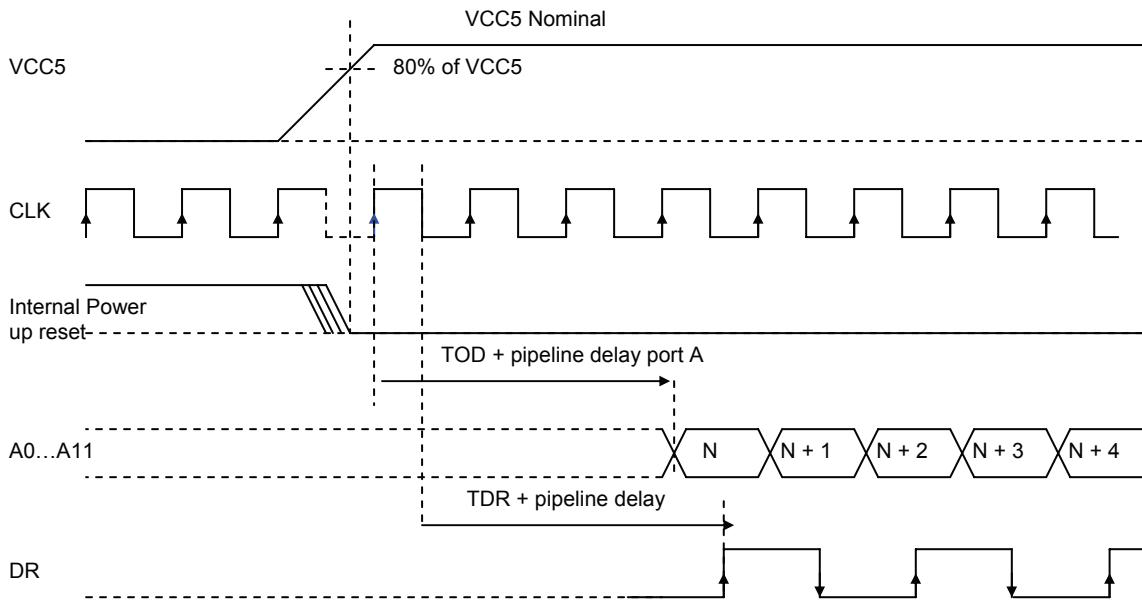
Figure 3 Power up reset Timing diagram (1:1 DMUX)
